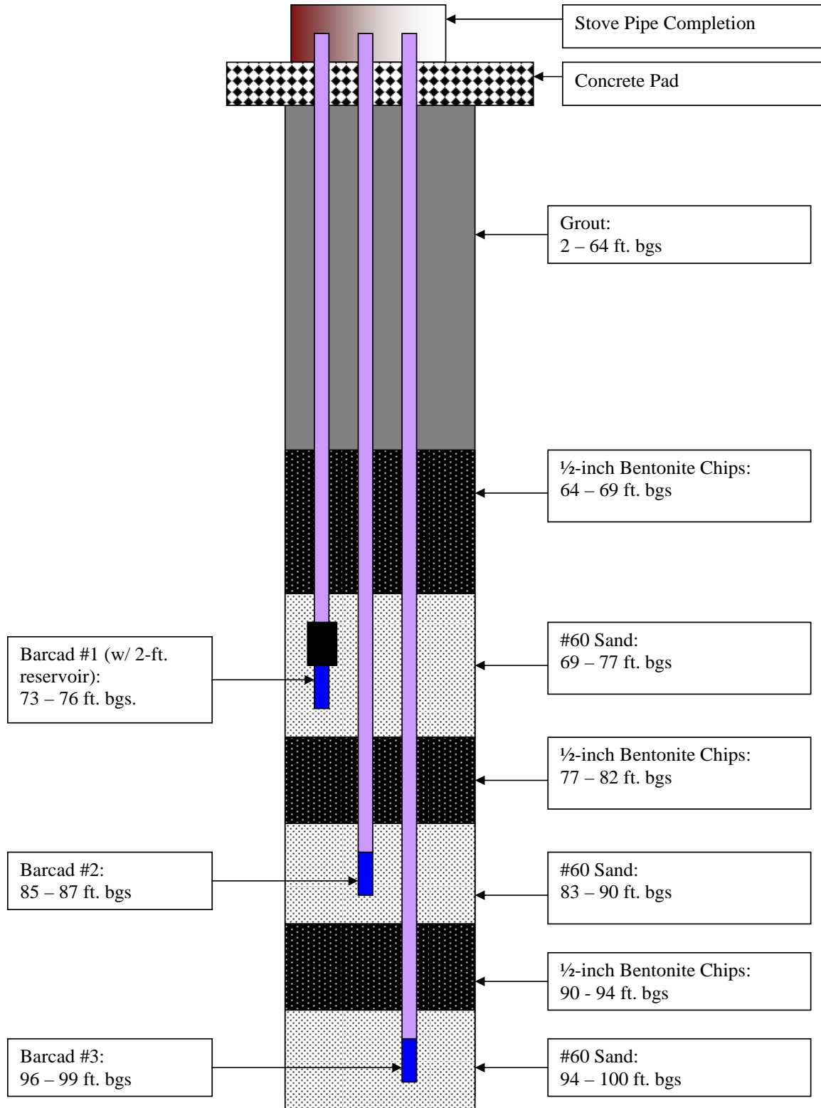
Figure 5: Buried Barcad nest. In unconsolidated to semi consolidated materials, the nest is installed through a temporary conductor casing provided by various drilling machines such as sonic, air rotary casing hammer, dual wall percussion, hollow stem auger. In hard rock and other types of competent materials, the Barcads can be buried directly into the borehole without a temporary conductor casing.
